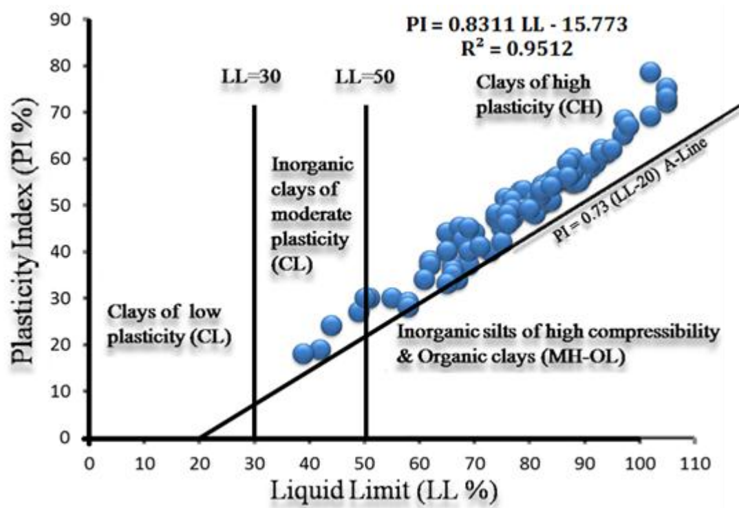
Fig. (2): Plasticity chart for the cohesive soils in Tanta City.
